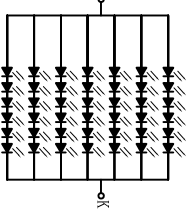
Backlight LED Circuit
