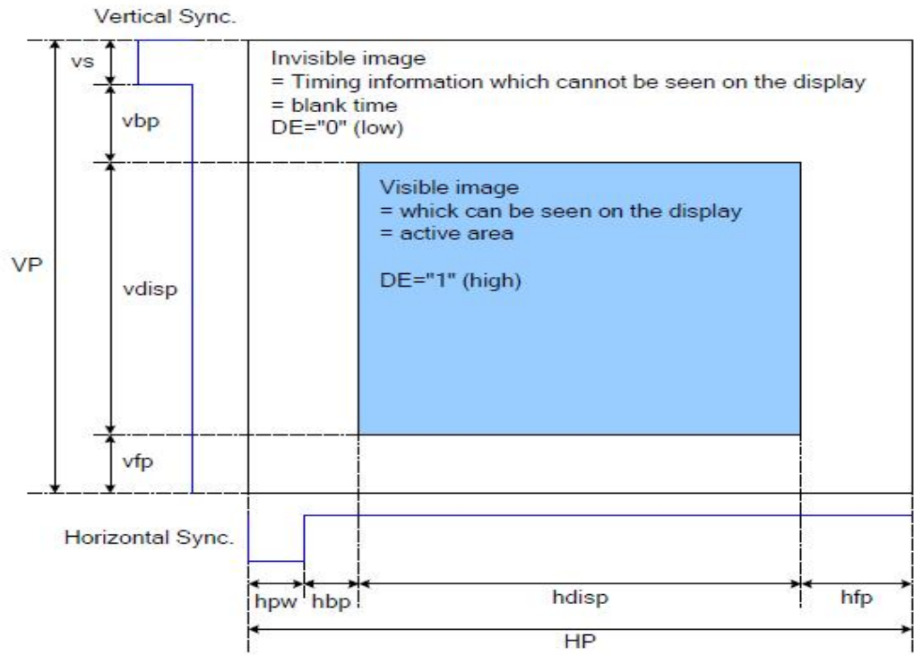
DRAM Access Area by RGB Interface
