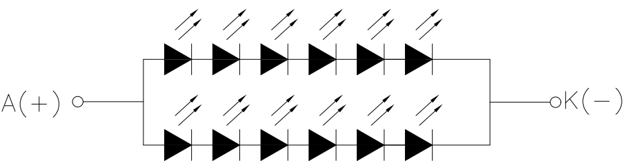
LED (B/L) CIRCUIT
