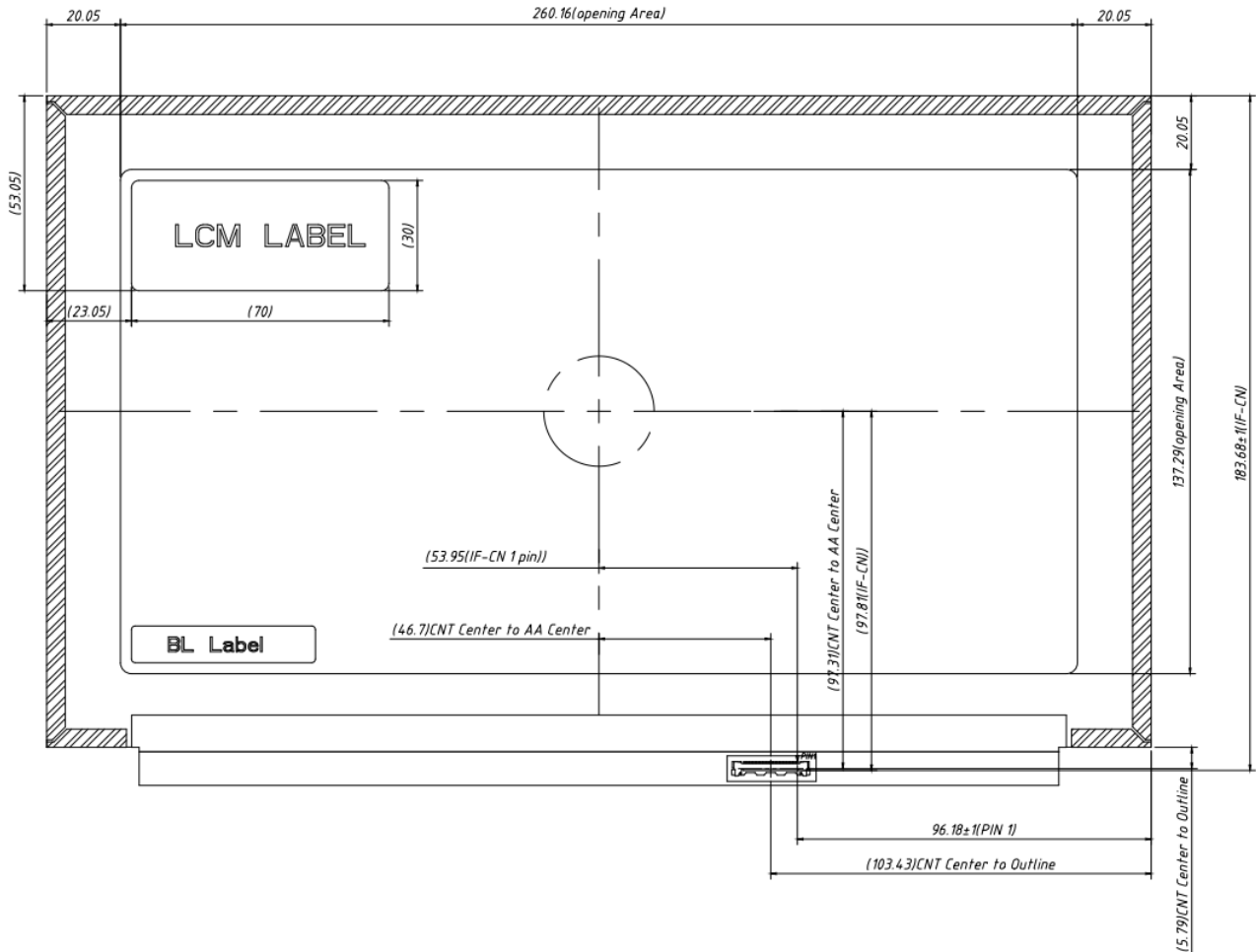
Figure 16 Reference Outline Drawing (Back Side)
