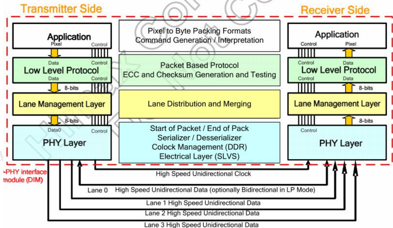
Figure 4.6: DSI transmitter and receiver interface
