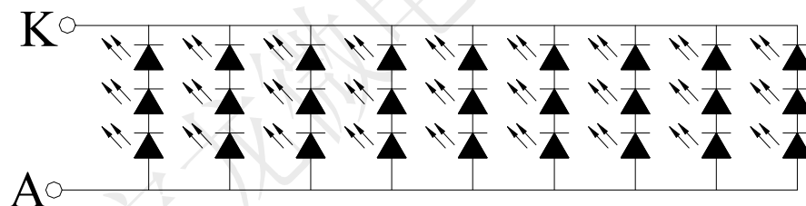
LED CIRCUIT DIAGRAM V_f=9.0\text{V}-10.5\text{V}(I_f=9*20\text{mA})
