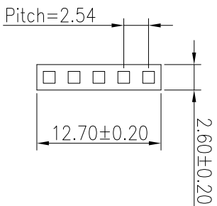
HOUSING
