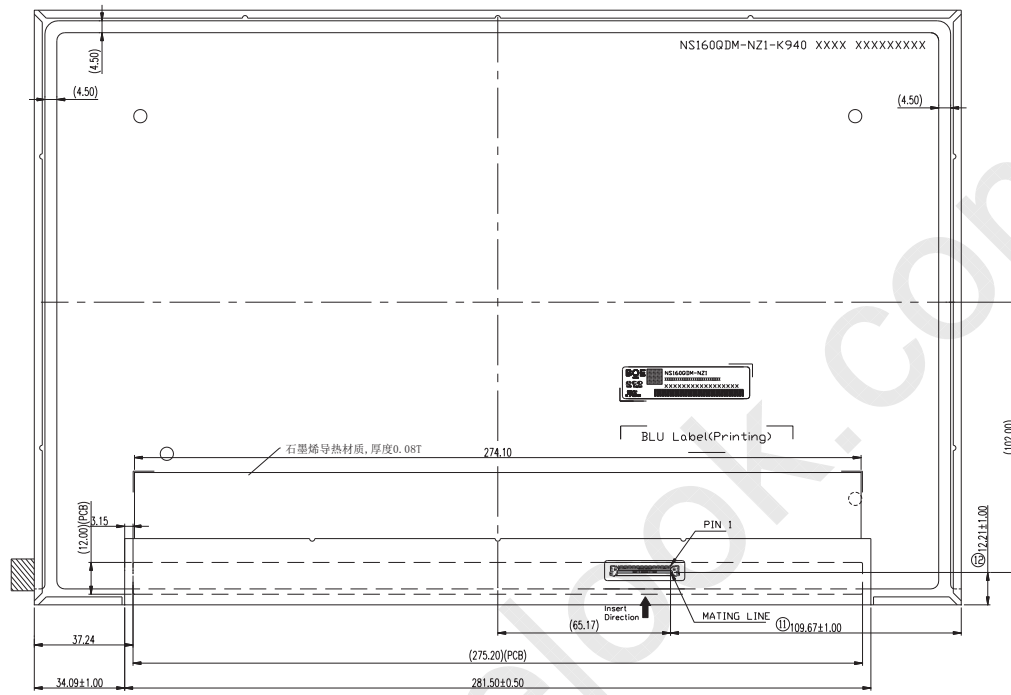
Figure 26. TFT-LCD Module Outline Dimensions (Rear view)
