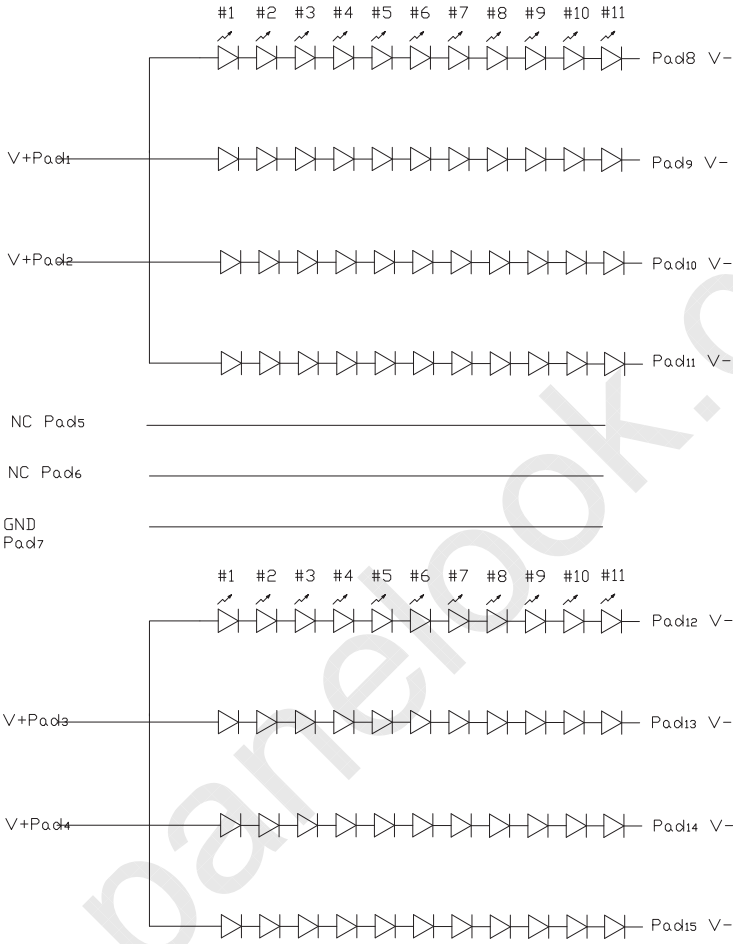
Figure 6. LED Structure
