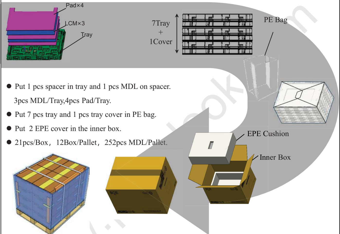
Figure 25. Packing Order
