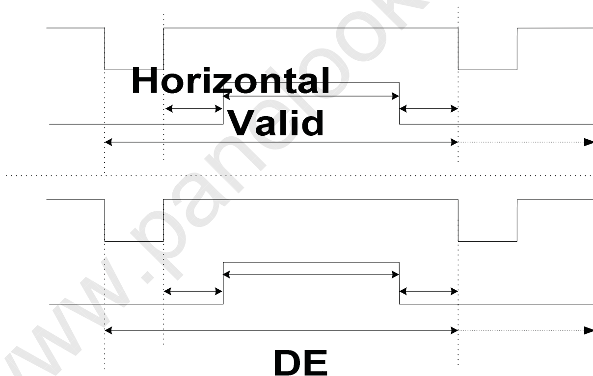
Fig.3-2 DE Mode Input Timing
