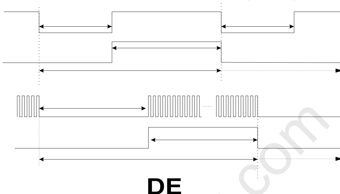
Fig.3-2 DE Mode Input Timing
